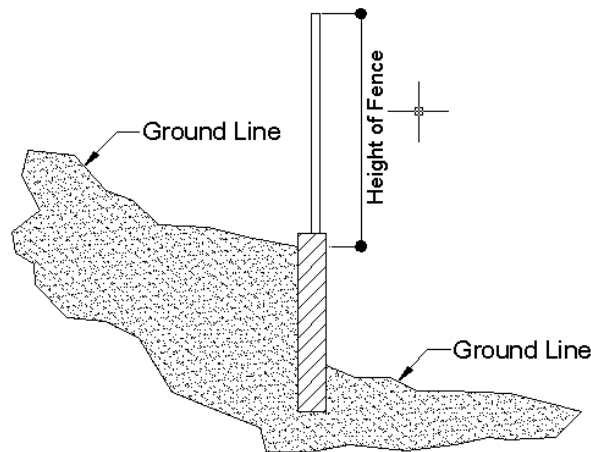
Fig. 3 Determining fence height
