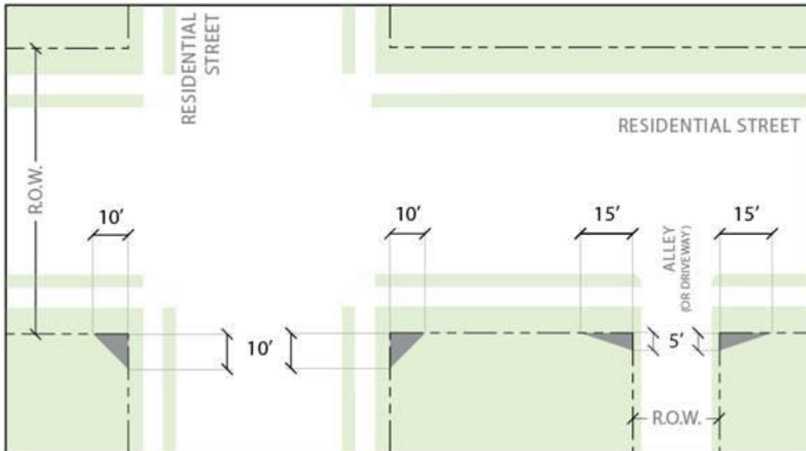
Fig. 1. Visibility Triangles
