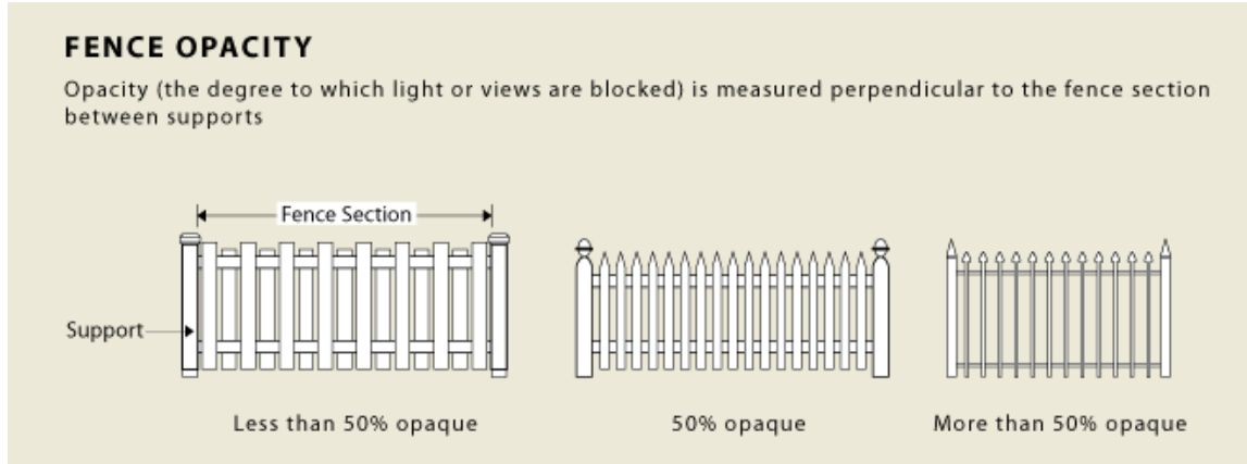
Fig 4. Opacity of fences
