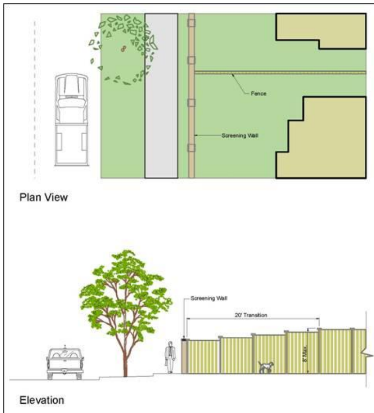
Fig. 2. Connecting to perimeter walls
